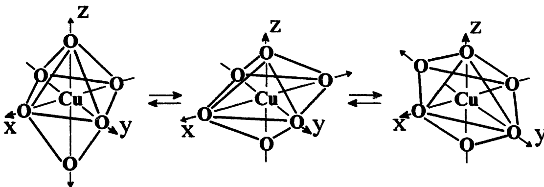
Fig. 3.6. Elongations along the three principal axes of the Cu–O bonds in the hexaaqua copper(II) complex due to dynamic Jahn–Teller effects occur randomly with a correlation time of about 5 \times 10^{-12} s.
