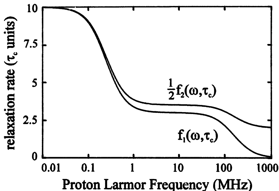
Fig. 3.10. Plot of f_1(\omega, \tau_c) and \frac{1}{2}f_2(\omega, \tau_c) of Eqs. (3.13) and (3.14) as a function of magnetic field (expressed as proton Larmor frequency; log scale). \tau_c = 2 \times 10^{-9} s.
